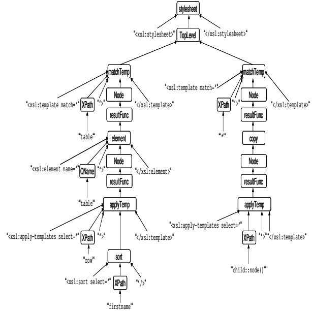
Figure 6: Abstract syntax tree of the XSLT stylesheet of Figure 1
