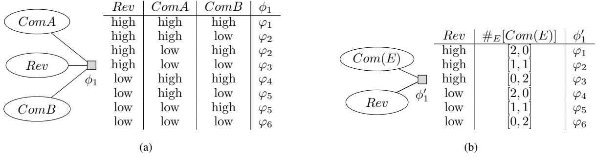
Figure 6: (a) An FG modelling the interplay between the revenue Rev of a company and the competences ComA and ComB of its employees, and (b) a lifted representation, encoded as a PFG, of the FG shown in (a). For brevity, we omit the argument lists of \phi_1 and \phi'_1 and write \phi_1 instead of \phi_1(Rev, ComA, ComB) and \phi'_1 instead of \phi'_1(Rev, \#_E[Com(E)]) .
