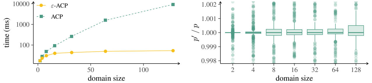
Figure 3: Average query times of lifted variable elimination on the output of ACP and \epsilon -ACP for every choice of k (left), and a boxplot showing the distribution of the quotient p'/p , where p' = P_{M'}(r | e) and p = P_M(r | e) , for each choice of k (right).
