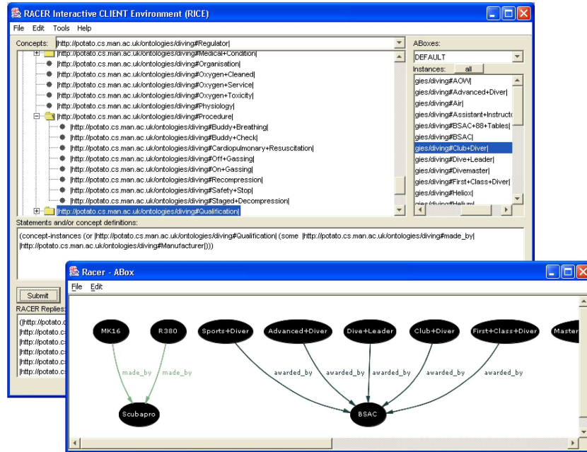
Fig. 3. Using RICE on the fly to visualize an RDF document interactively defined with OilEd.
