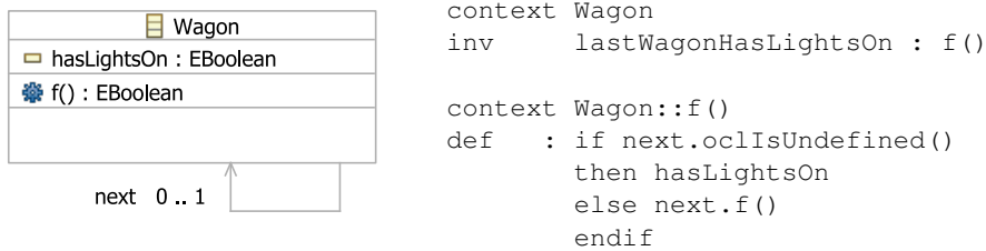
Figure 3: An example where data accesses traverse links known only at runtime
